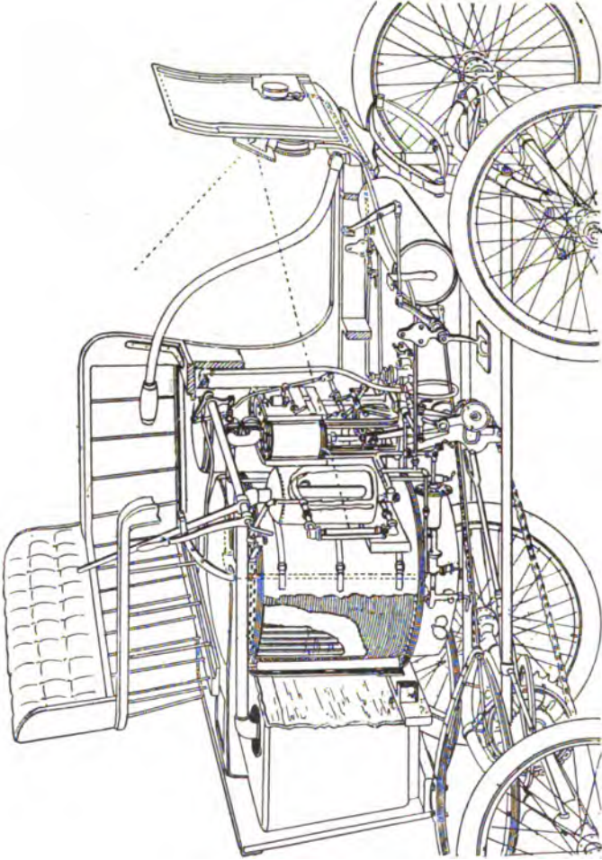
FIG. 244.—Part sectional view of the "Locomobile" Steam Carriage, showing machinery and parts in position.
